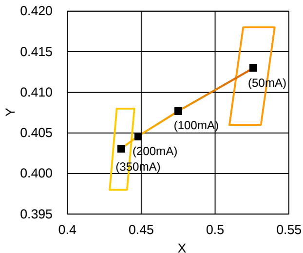
Fig 7. Chromaticity Coordinate Profile at T_C=25^\circ\text{C} .
